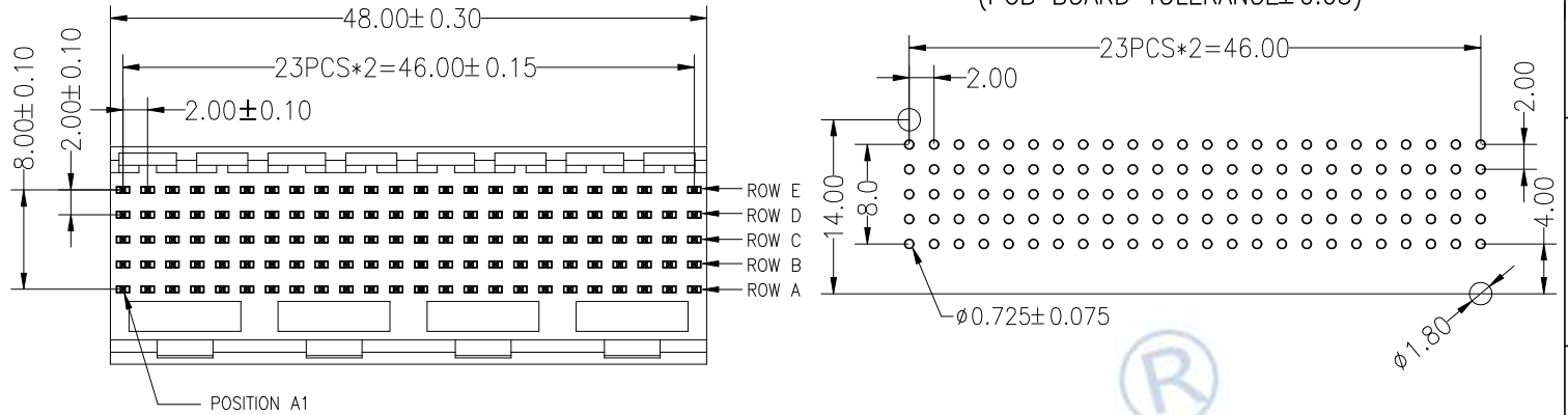
Recommended P.C.B Layout(Top Side) (PCB BOARD TOLERANCE±0.05)
