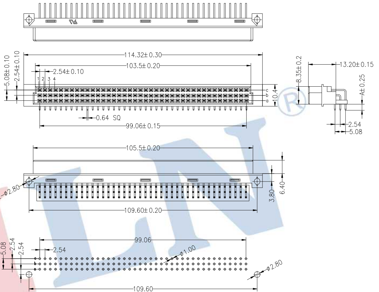
Recommended P.C.B Layout(Top Side) (PCB BOARD TOLERANCE± 0.05)
